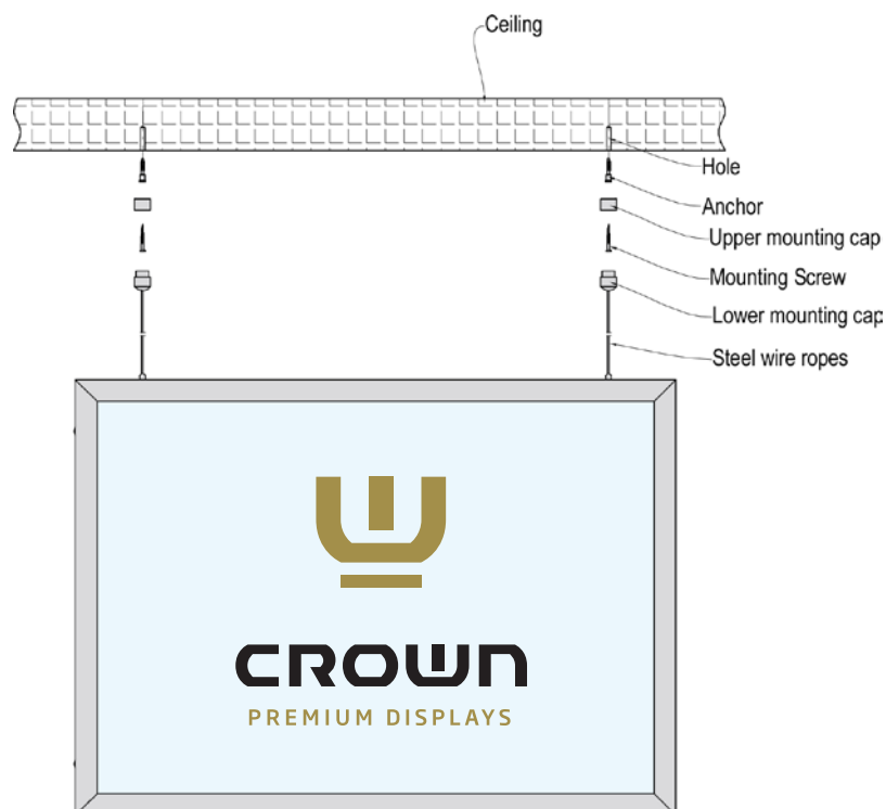
Assembly of the ceiling mounting apparatus
